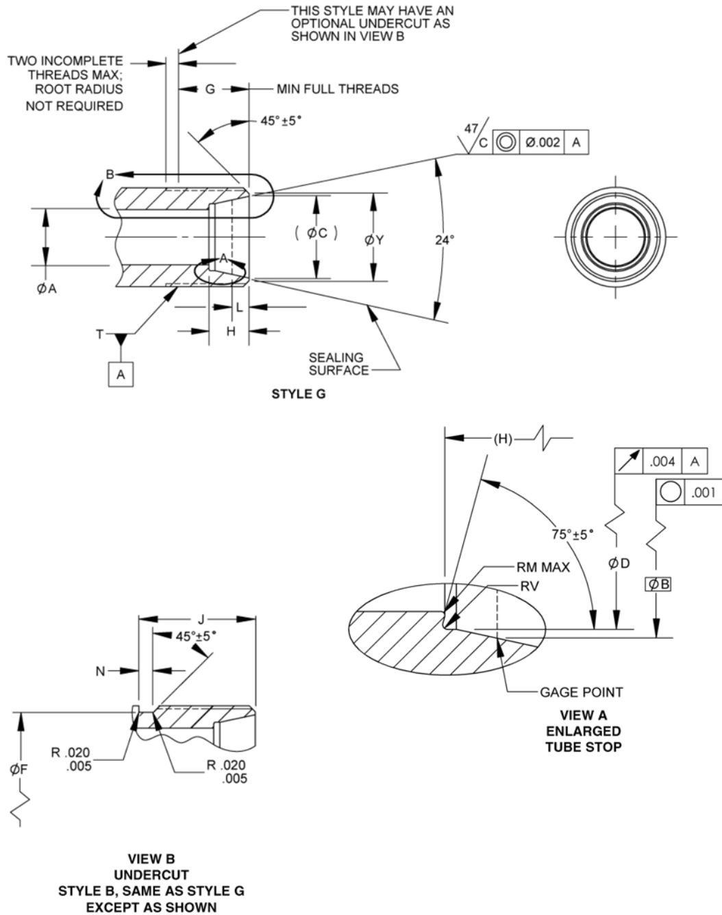
FIGURE 1 - FITTING END DESIGN, STYLES B AND G
