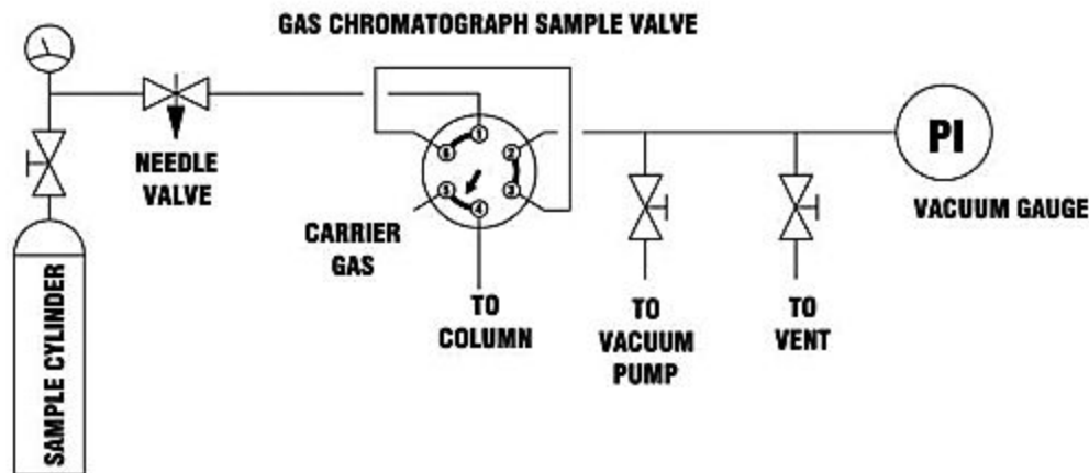
FIG. 1 Suggested Manifold Arrangement for Entering Vacuum Samples
